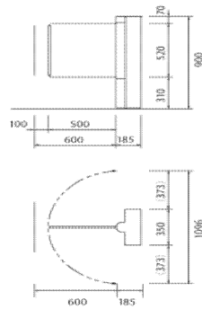
■ Single flap-panel specifications
