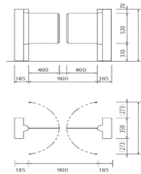
■ Double flap-panels specifications
